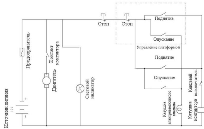
2. Electric principal Scheme
